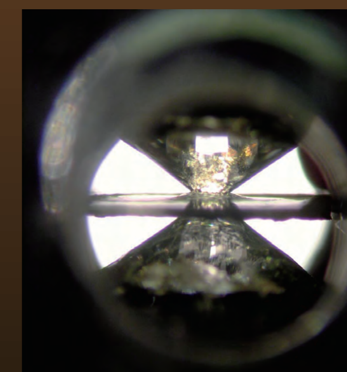
Diamond anvil apparatus: High pressure and high temperature beyond the center of the Earth can be achieved.
