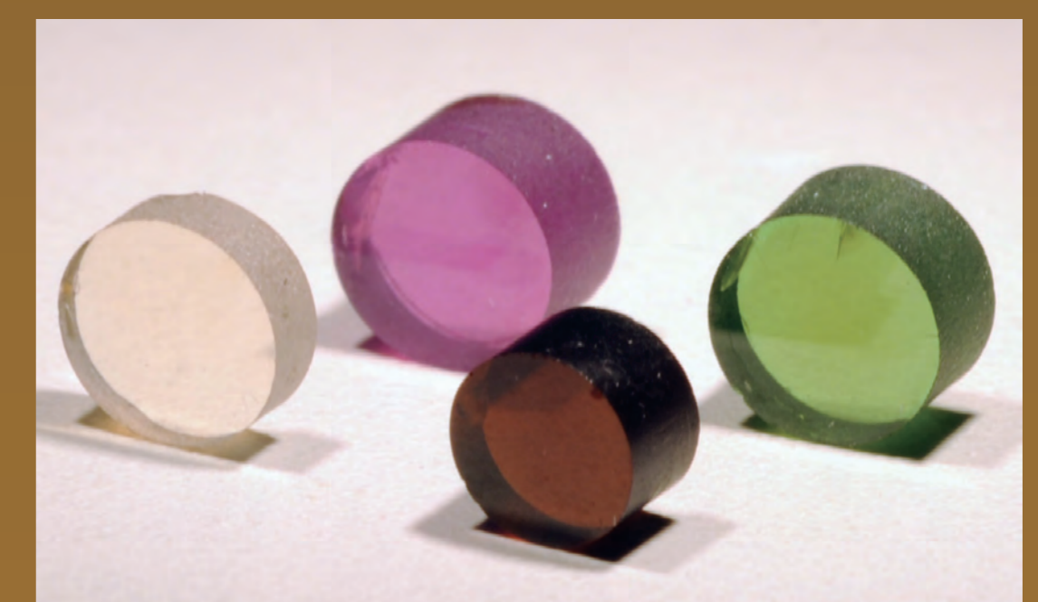
Nano-polycrystalline garnet
